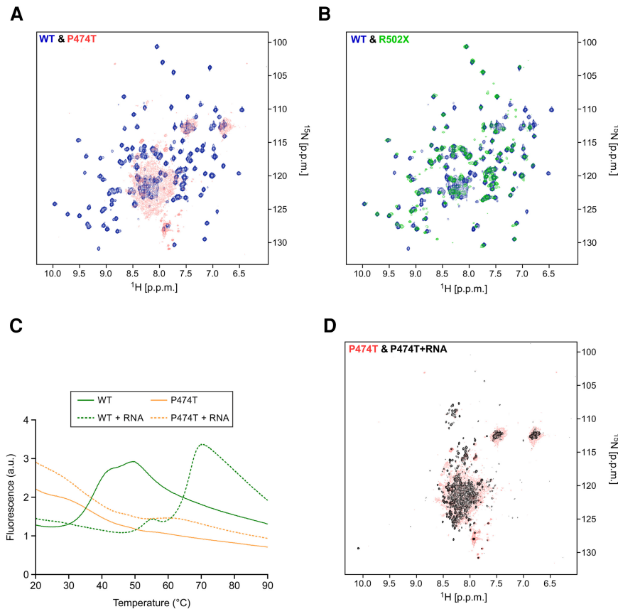
FIGURE 6. Stability and folding properties of 65K C-RRM and its P474T and 502X variants. (A) An overlay of the [ ^1\text{H} , ^{15}\text{N} ]-HSQC spectra of the wild-type 65K C-RRM (blue) and P474T 65K C-RRM (pink). (B) An overlay of the [ ^1\text{H} , ^{15}\text{N} ]-HSQC spectra of the wild-type 65K C-RRM (blue) and R502X 65K C-RRM (green). (C) Differential scanning fluorimetry analysis of wild-type and P474T-mutant RRM domain. Melting curves of untagged wild-type and P474T-mutant RRM were obtained in the absence or presence of U12 RNA oligonucleotide by heating the proteins or protein–RNA complexes in the presence of SYPRO Orange and recording the fluorescence of the dye as a function of temperature. (D) An overlay of the [ ^1\text{H} , ^{15}\text{N} ]-HSQC spectra of 65K C-RRM (P474T) in the absence (pink) and presence of RNA (black).
