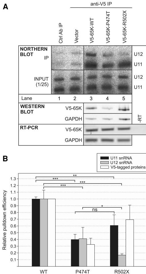
FIGURE 2. 65K mutants form di-snRNP with reduced efficiency. (A) HeLa cells were transfected with plasmids for expressing V5-tagged 65K protein (WT, P474T, or R502X) or empty vector. After cell lysis, immunoprecipitation was carried out using either anti-V5 antibody or anti-FLAG antibody as a control for nonspecific binding and co-immunoprecipitation of U11 and U12 snRNAs was analyzed by northern blot. Protein and mRNA level measurements of exogenous 65K by western blotting and RT-PCR, respectively, were carried out from experiments run parallel with the co-IP samples. (B) Quantification of the northern (co-IP) and western blot data from A. U11 and U12 co-IP data were derived from three independent experiments which were normalized within each experiment by setting the mean U11 + U12 value of the WT co-IP reaction to one. V5-tagged protein level measurements were similarly derived from three independent experiments and normalized first using GAPDH signal, then by setting the WT value to one. Significance levels are indicated (ns: P > 0.05 , [*] P \leq 0.05 , [**] P \leq 0.01 , [***] P \leq 0.001 ).
