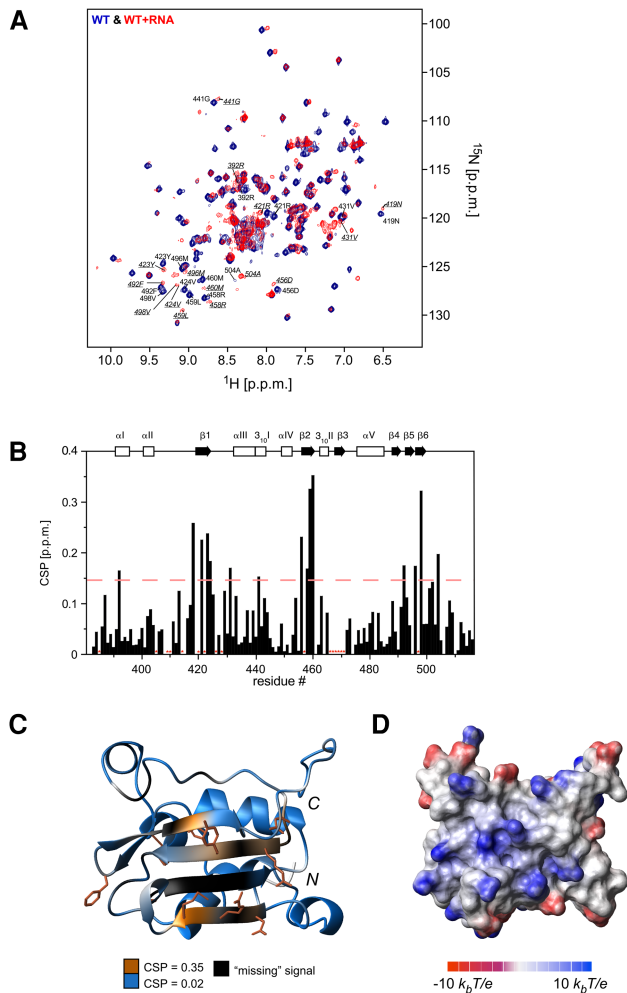
FIGURE 5. Interactions between wild-type 65K C-RRM domain and U12 RNA. (A) An overlay of the ^{1}\text{H} , ^{15}\text{N} -HSQC spectra of wild-type 65K C-RRM in the absence (blue) and presence of U12 RNA (red). The residues with significant chemical shift perturbations (>0.15) are labeled in both spectra. The residues that could not be unambiguously identified in the ^{1}\text{H} , ^{15}\text{N} -HSQC spectrum of the C-RRM/RNA complex are indicated with asterisks in red. The regions of the secondary structures are indicated above the plot. (B) A plot of chemical shift perturbation versus the residue number. The dashed line represents the threshold used as the criteria for significant chemical shift perturbations. The residues that could not be unambiguously identified in the ^{1}\text{H} , ^{15}\text{N} -HSQC spectrum of the C-RRM/RNA complex are indicated with asterisks in red. The regions of the secondary structures are indicated above the plot. (C) Chemical shift perturbations are mapped on the wild-type 65K C-RRM structure, where blue color indicates smallest and orange biggest CSP value. Locations with the missing signals in ^{1}\text{H} , ^{15}\text{N} -spectrum of the wild-type 65K C-RRM/RNA complex are colored black. Prolines and other unassigned residues are colored in white. Side-chains of the residues with larger chemical shift perturbations (>0.15) are displayed by stick models. (D) Surface electrostatic potential of wild-type 65K C-RRM is shown as a colored gradient between -10 k_b T/e and 10 k_b T/e , where k_b is Boltzmann's constant, T temperature, and e elementary charge. The structures are visualized by MOLMOL.
